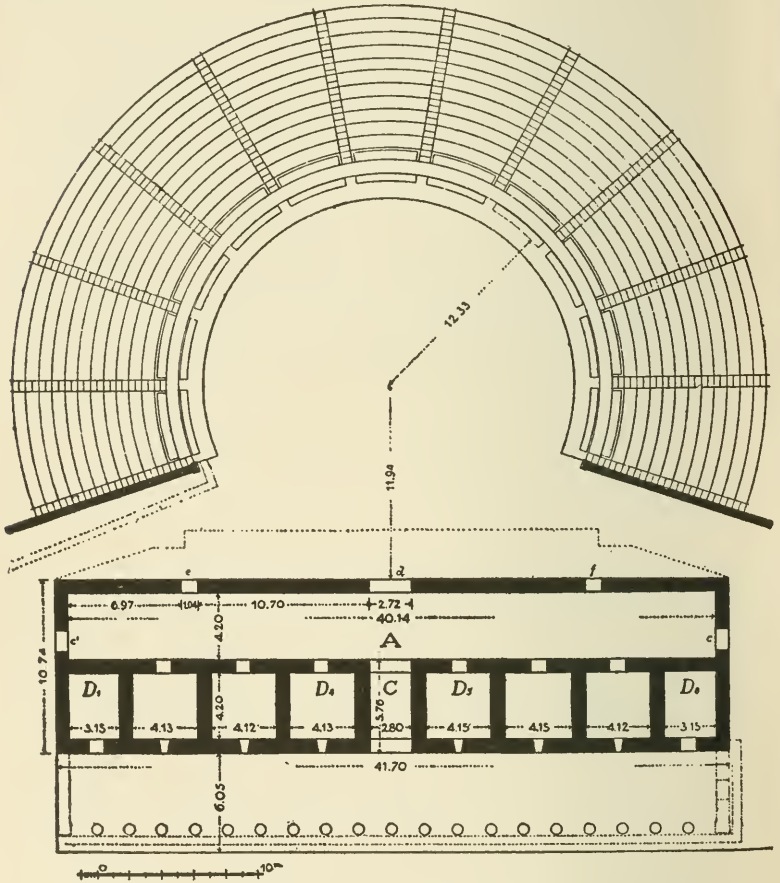
FIG. 60.—Ground Plan of the Early Hellenistic Theater at Ephesus
